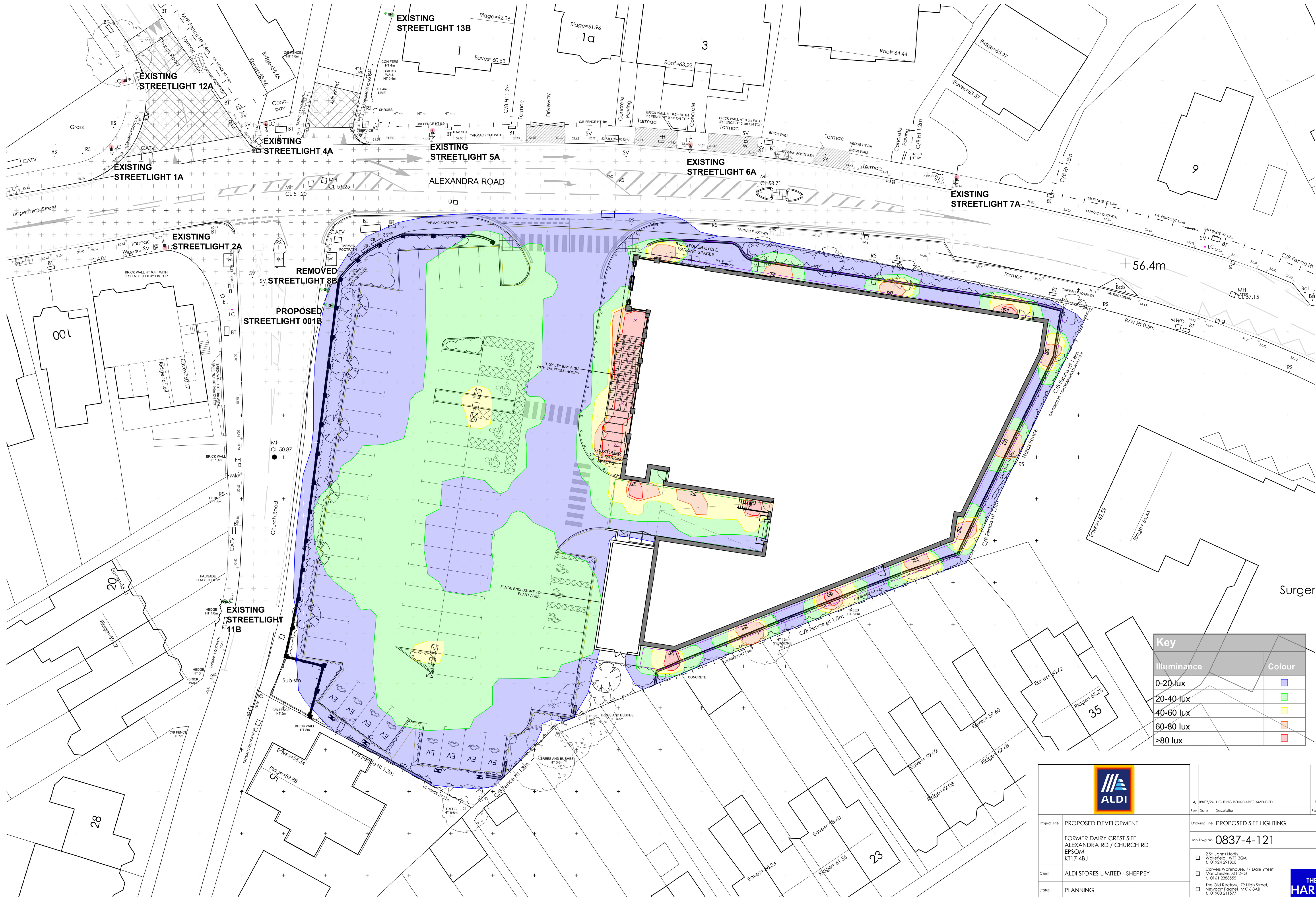
01 PROPOSED SITE LAYOUT 1:200
