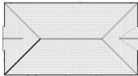
9 Proposed Roof Plan 1:100
