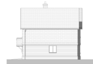
7 Side Elevation 2 1 : 100
