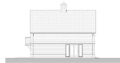
7 Side Elevation 2 1 : 100
