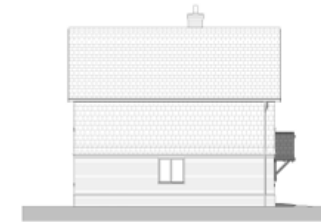
5 Side Elevation 1 1 : 100
